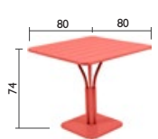
GUÉRIDON PEDESTAL TABLE Aluminium Aluminium 19.6 kg
