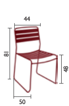
CHAISE CHAIR
